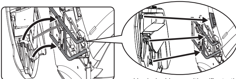
Hook docking position illustration
